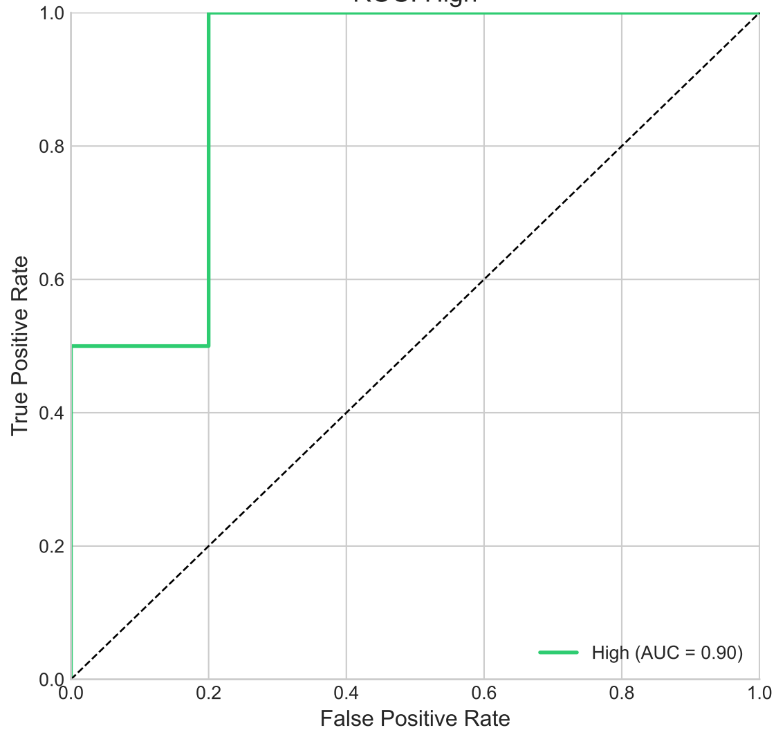
ROC: High
