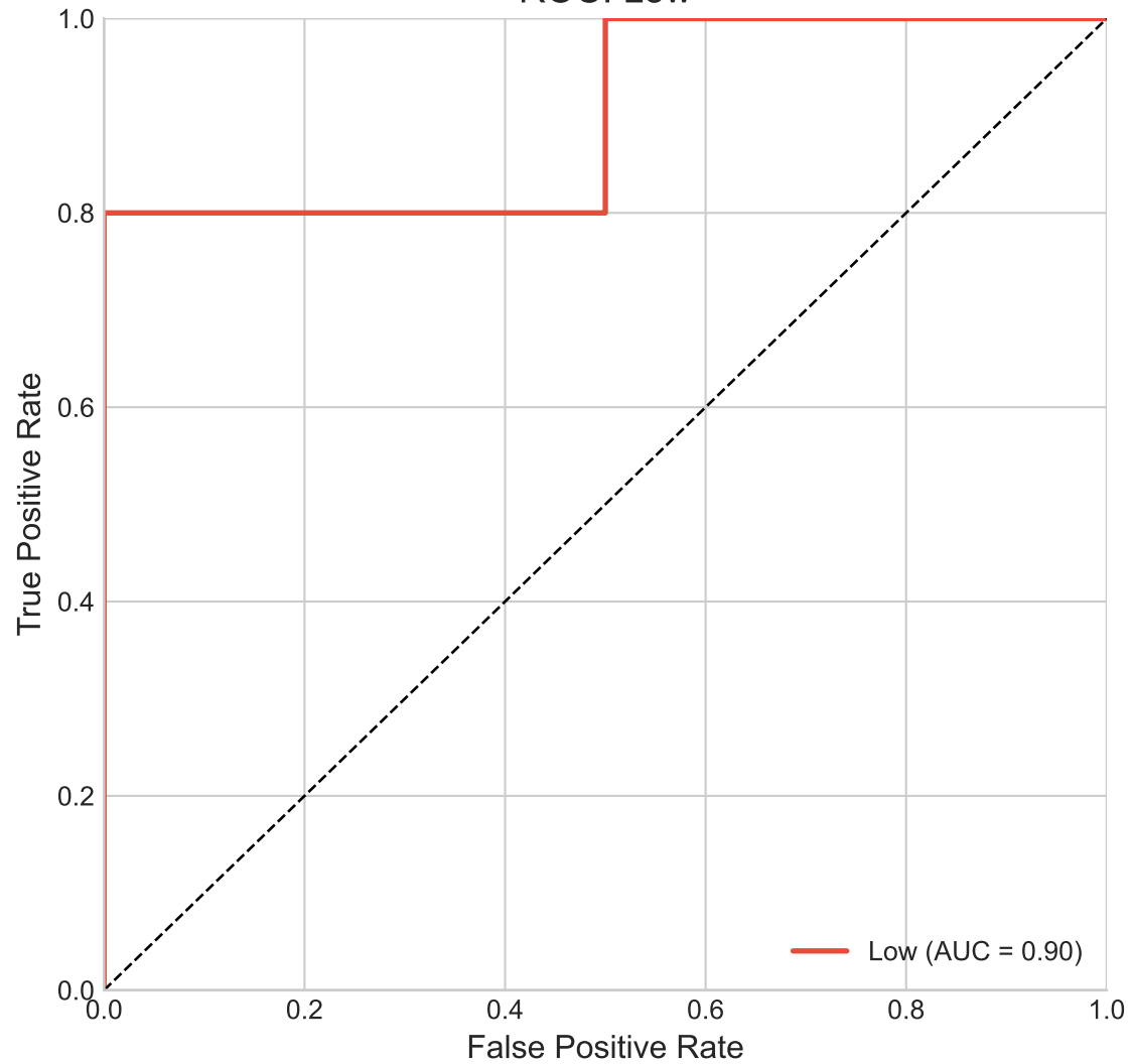
ROC: Low
